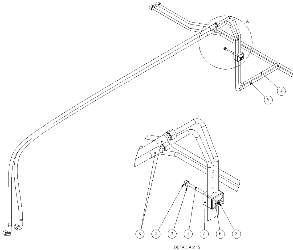
DETAIL A 2:5
